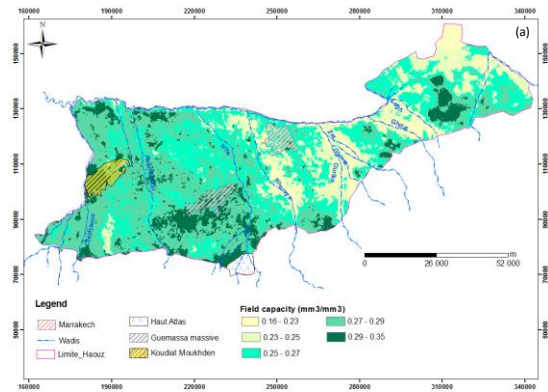
The spatial variation of moisture soil at Field capacity ( \theta_{fc} ) over Haouz plain at 100 m spatial resolution
